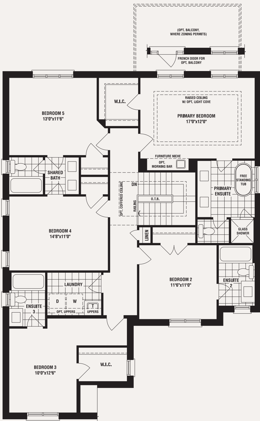
EXPANDED LIVING 5TH BEDROOM OPTION
