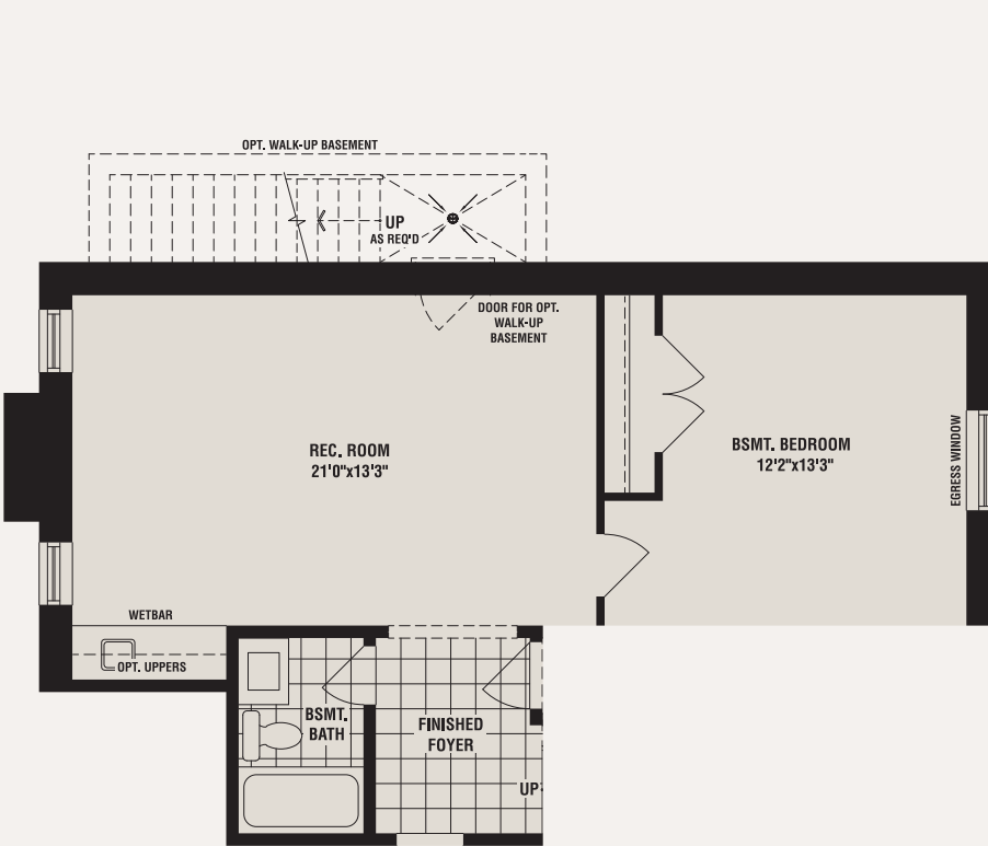
FAMILY FLEX SUITE OPTION +719 SQ. FT.
